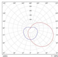
LOUVRE
